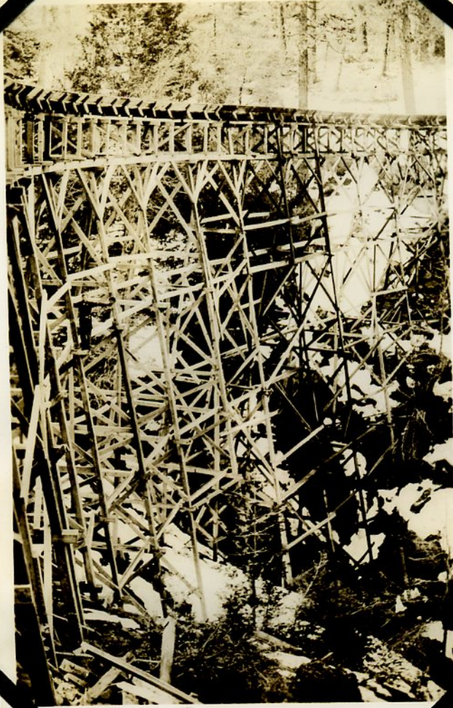
Pine Ridge flume across Musick Creek - (Photo #50)
